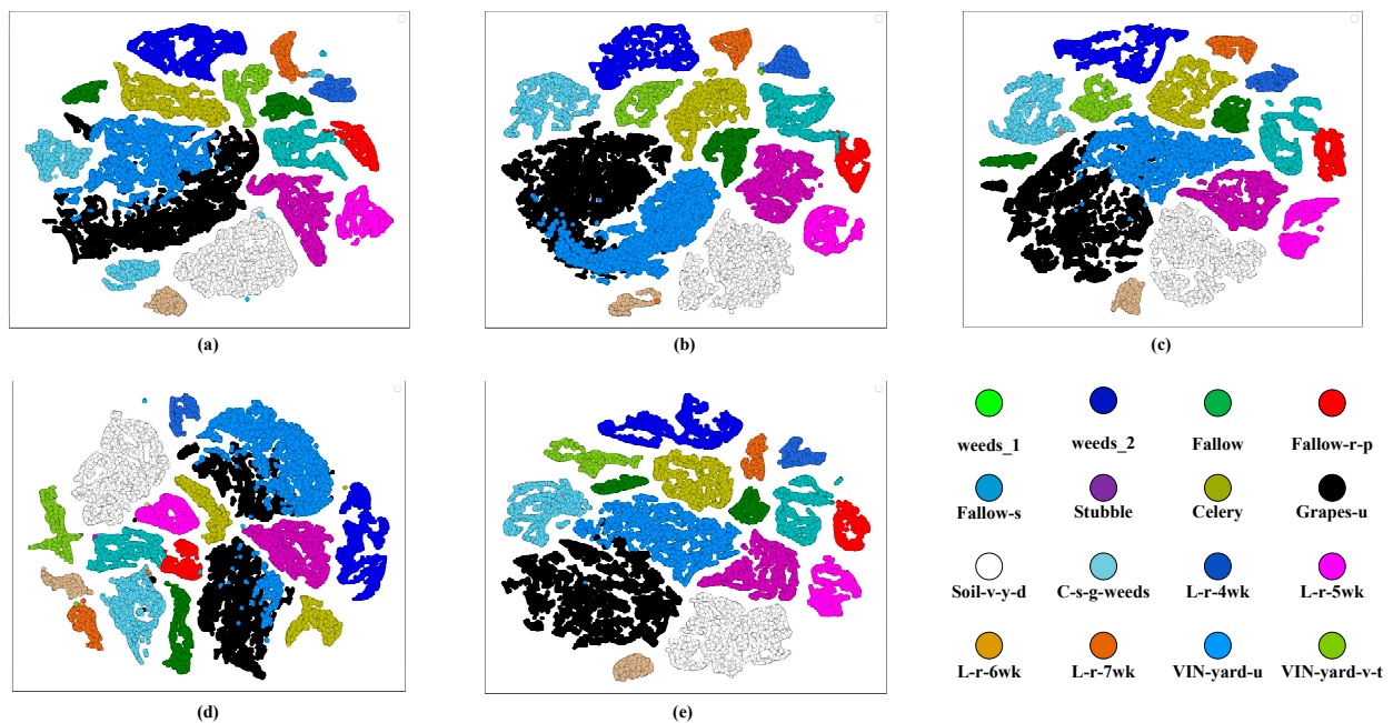
Figure 16. Visualization of feature separability for different methods on SV. (a) DBDA, (b) FECNet, (c) FDSSC, (d) DTAN, (e) Proposed.
