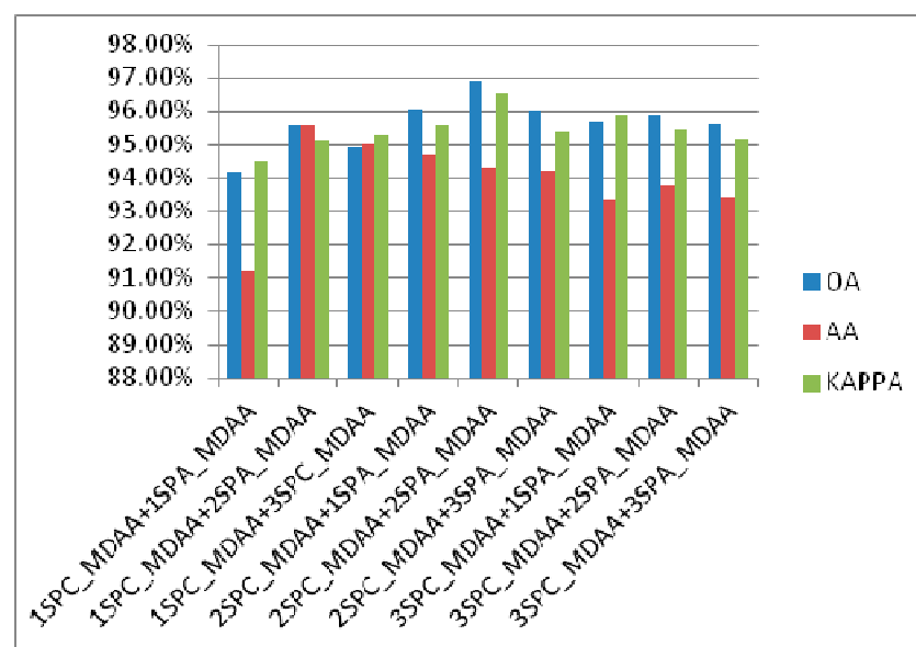
Figure 8. Classification accuracy of different combinations of the SPA_MDAA and the SPE_MDAA in IN.
