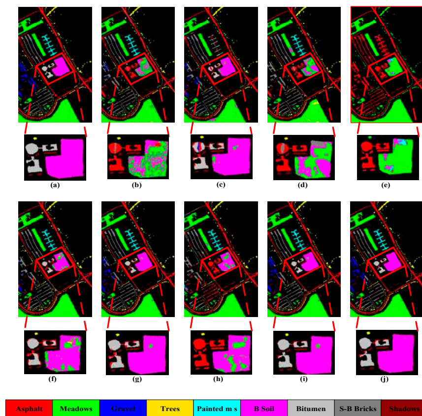
Figure 12. Classification maps on UP dataset, (a) ground truth, (b) SVM, (c) SSRN, (d) FDSSSC, (e) CDCNN, (f) DBMA, (g) DBDA, (h) DTAN, (i) FECNet, (j) proposed.
