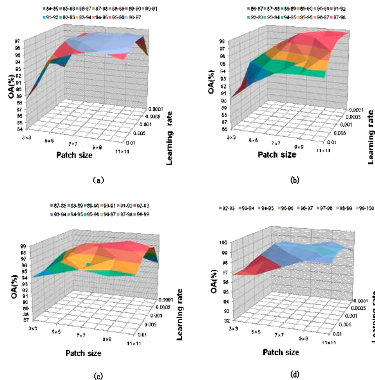
Figure 7. Effect of input patch size on accuracy at different learning rate. (a) IN, (b) SV, (c) UP, (d) KSC.
