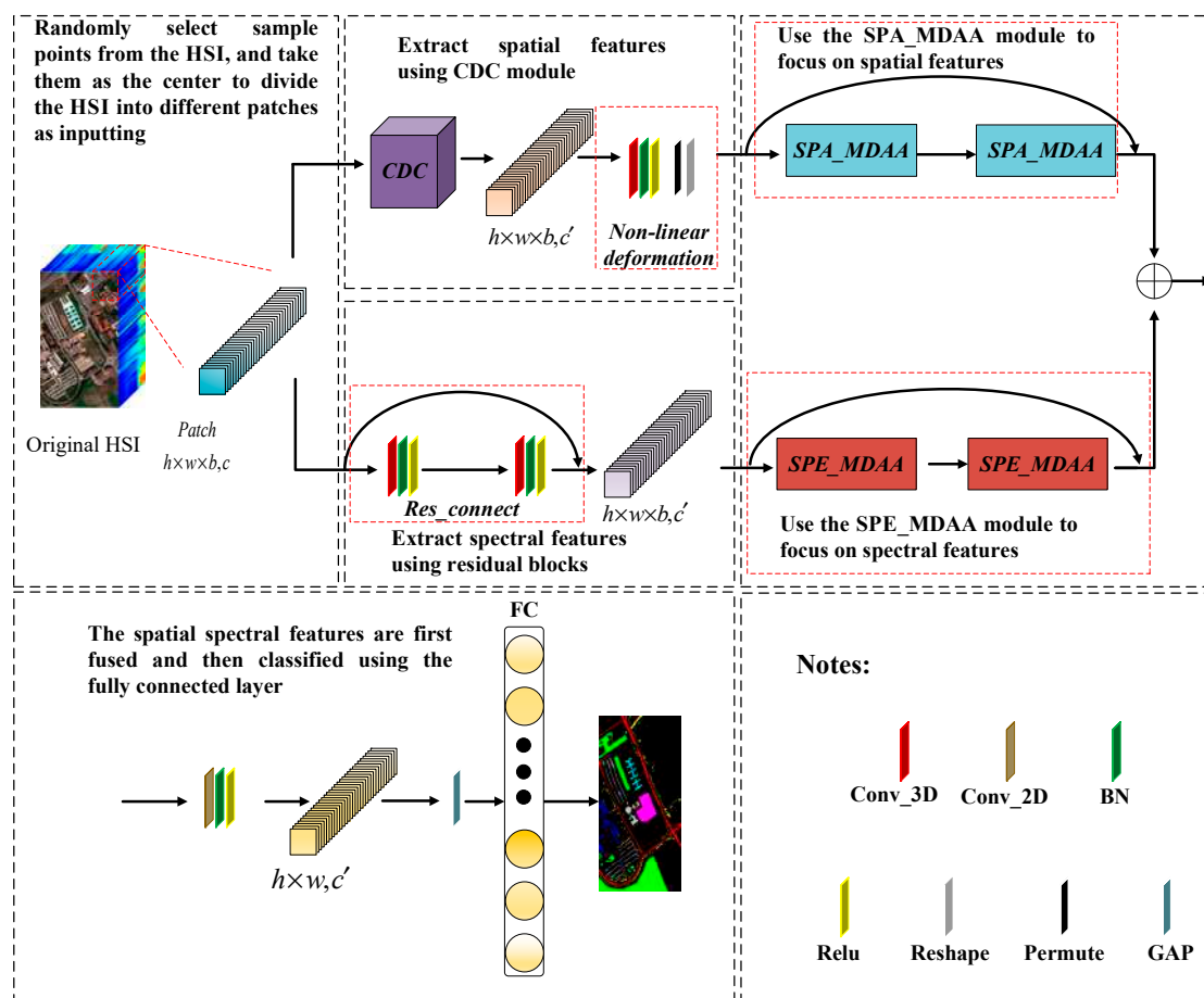
Figure 1. The overall structure of CDC_MDAA.
