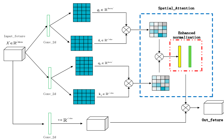
Figure 3. The SPA_DAA module.
