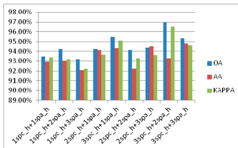
Figure 9. Classification accuracy of CDC_MDAA with different number of headers on IN dataset.
