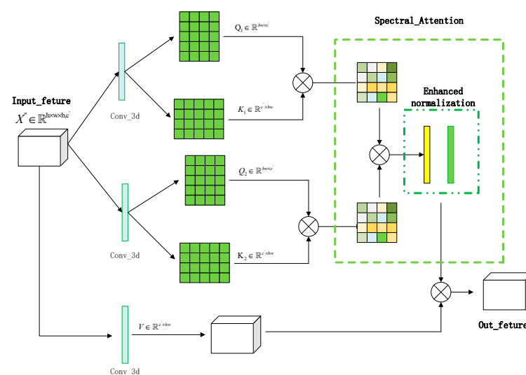
Figure 4. The SPE_DAA module.
