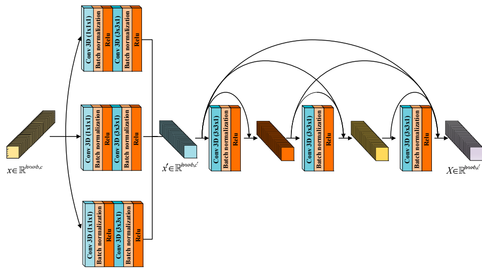
Figure 2. The CDC module.
