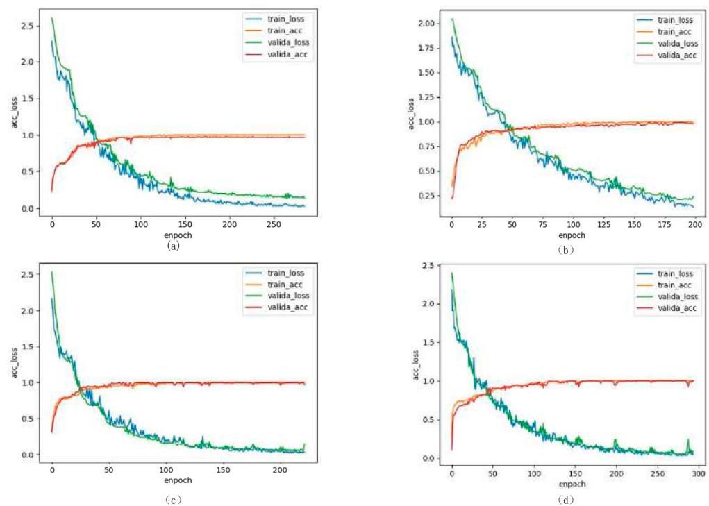
Figure 10. (a) training loss, training accuracy, verification loss, and verification accuracy on IN dataset, (b) training loss, training accuracy, verification loss, and verification accuracy on UP dataset, (c) training loss, training accuracy, verification loss, and verification accuracy on SV dataset, (d) training loss, training accuracy, verification loss, and verification accuracy on KSC dataset.
