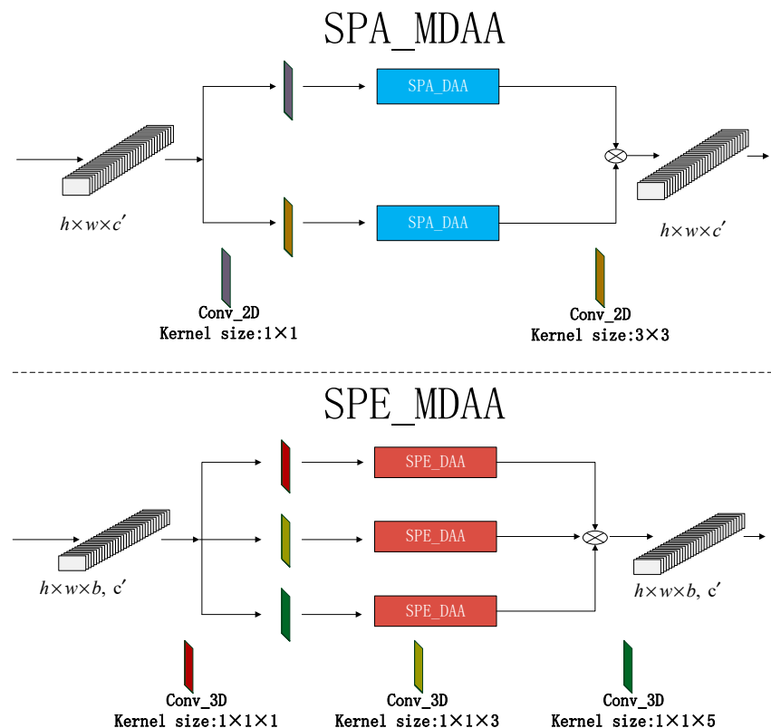
Figure 5. Multi-scale dual aggregated attention mechanism.
