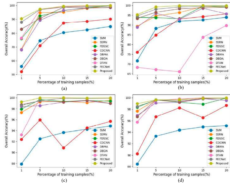
Figure 15. Classification results of all methods with different number of training samples on four data sets. (a) IN, (b) KSC dataset, (c) SV, (d) UP.
