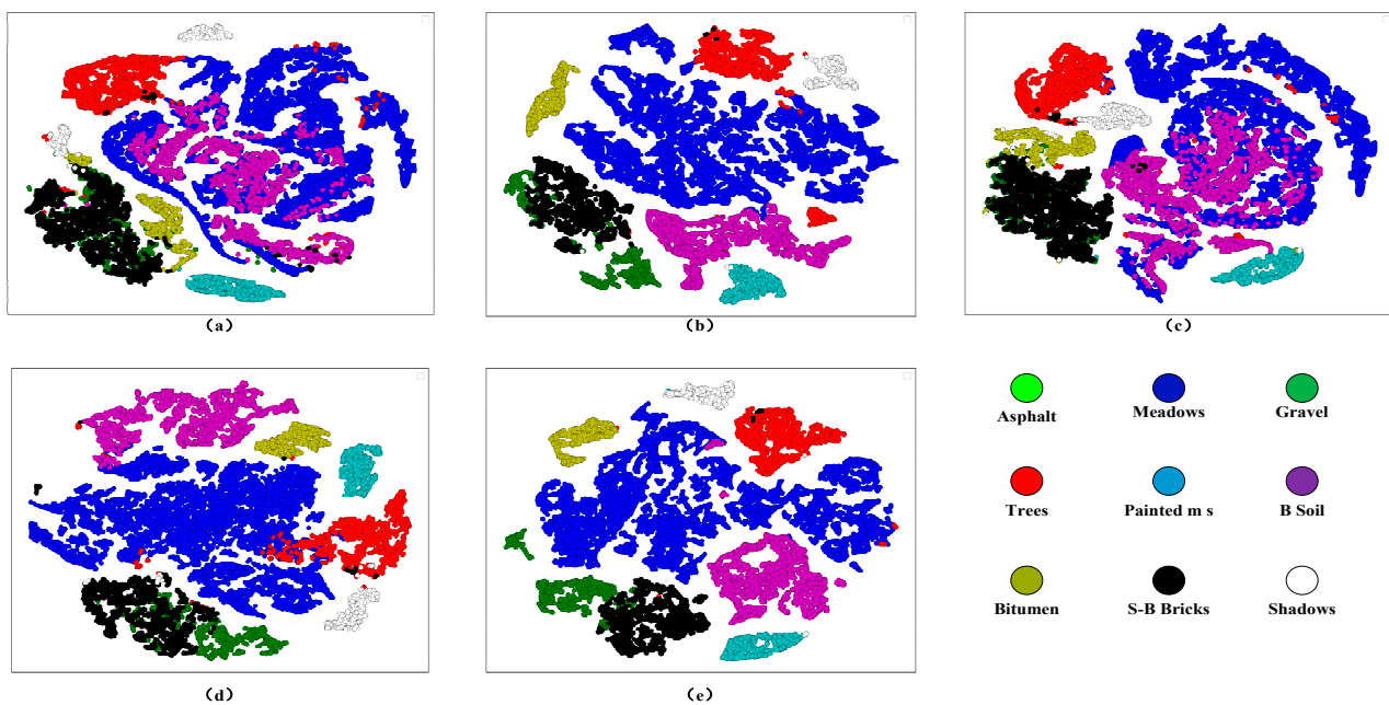
Figure 17. Visualization of feature separability for different methods on UP. (a) DBDA, (b) FECNet, (c) FDSSC, (d) DTAN, (e) Proposed.
